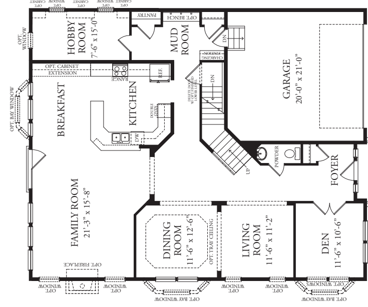
ALTERNATE FIRST FLOOR PLAN WITH HOBBY ROOM
