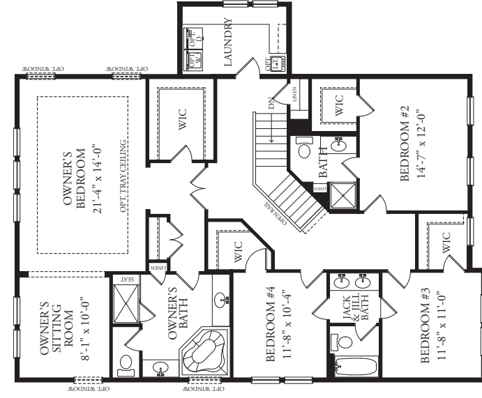
ALTERNATE SECOND FLOOR WITH OPT. LAUNDRY ROOM AND BEDROOM #2 SUITE
