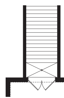
OPT. AREAWAY OR WALK-OUT
