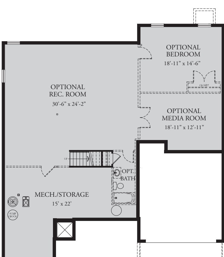
PARTIAL FOUNDATION PLAN W/ OPT. DOUBLE WELLED EXIT COND.
