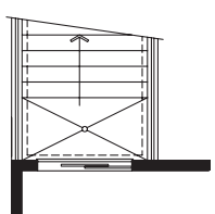
PARTIAL FOUNDATION PLAN W/ OPT. DOUBLE WELLED EXIT COND.
