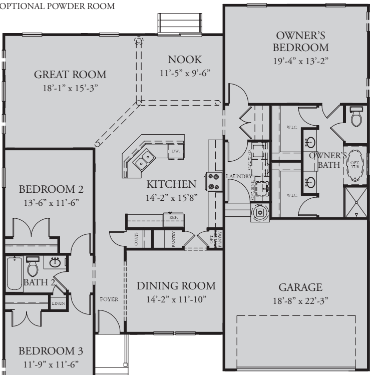
BASE PLAN
